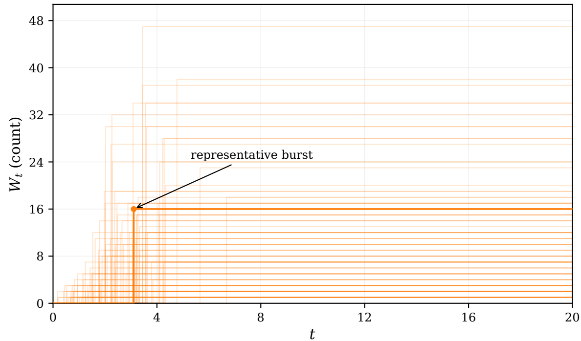
100 Gillespie realisations of W_t
